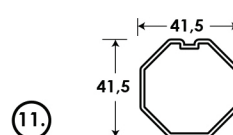
Int. Tube Drive Shaft profile
